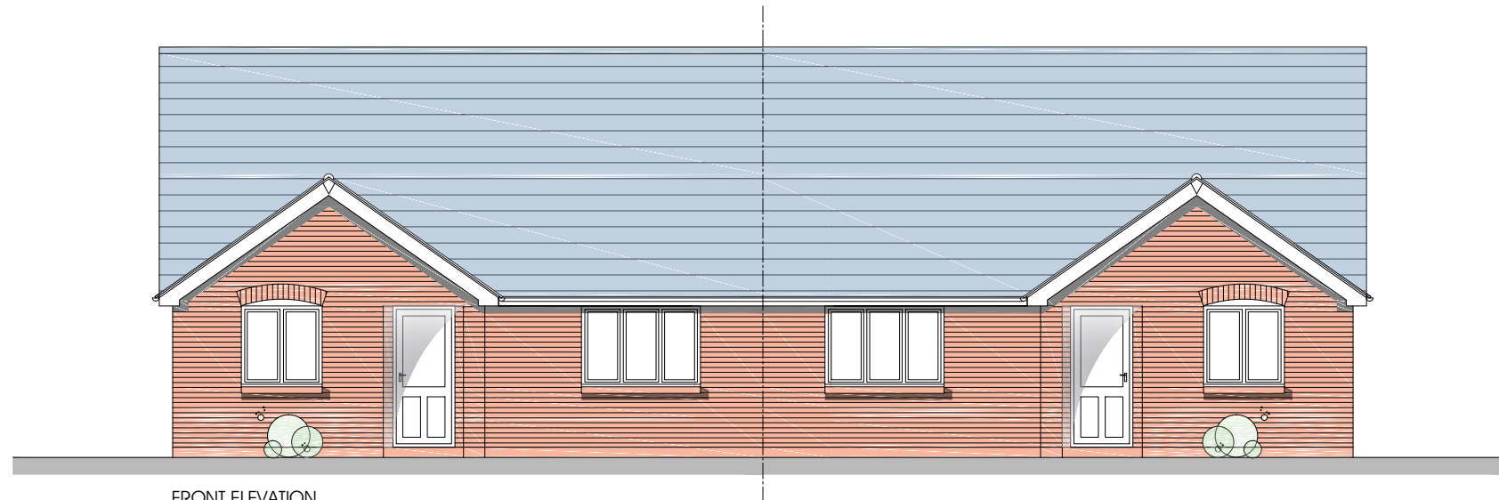
FRONT ELEVATION Typical 2 Bed Bungalow
